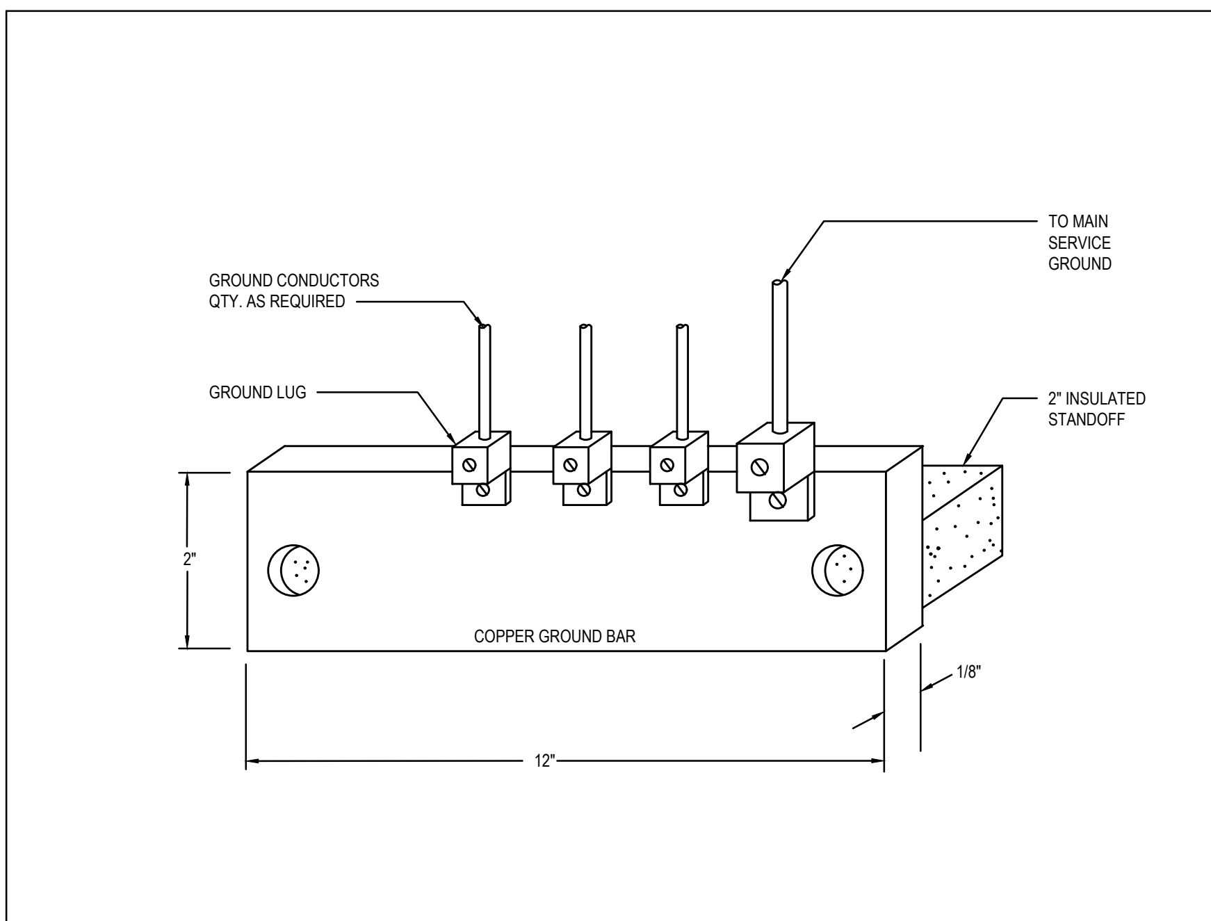
COMMUNICATIONS GROUND BAR DETAIL
