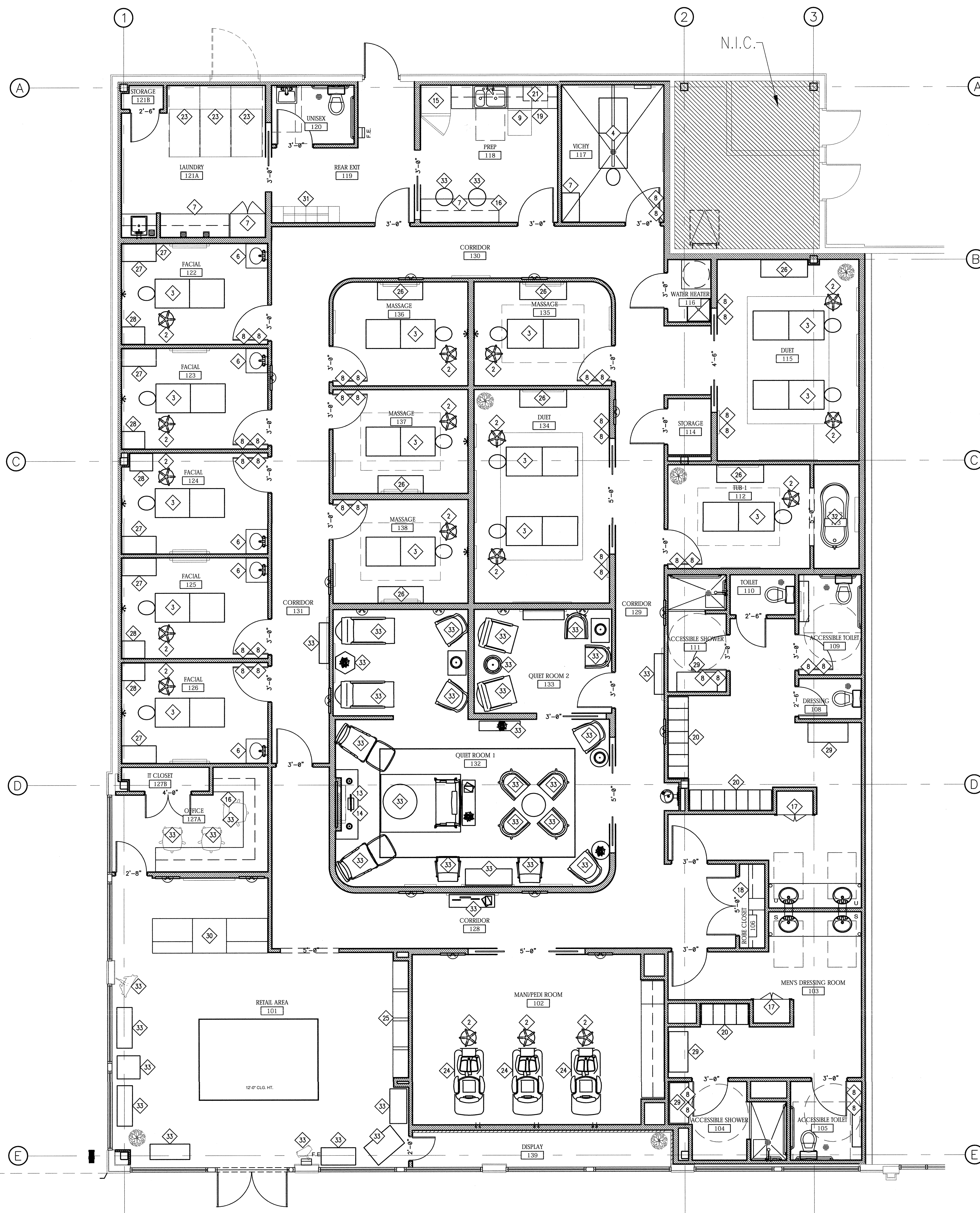
1 FURNITURE & EQUIPMENT PLAN 1/4" = 1'-0" PLAN NORTH
